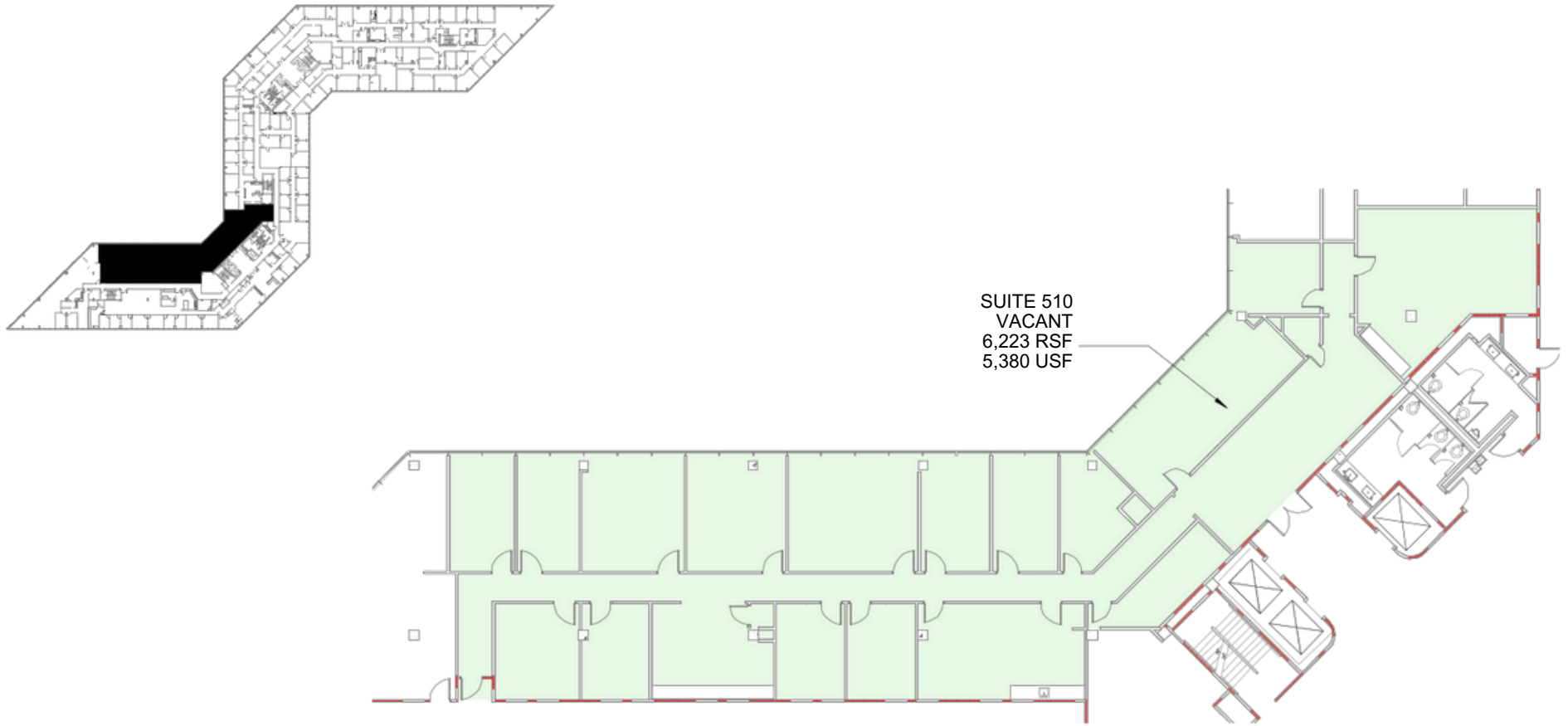
A1 PLAN 1/16" = 1'-0" LEVEL 5 -510 MP 510
